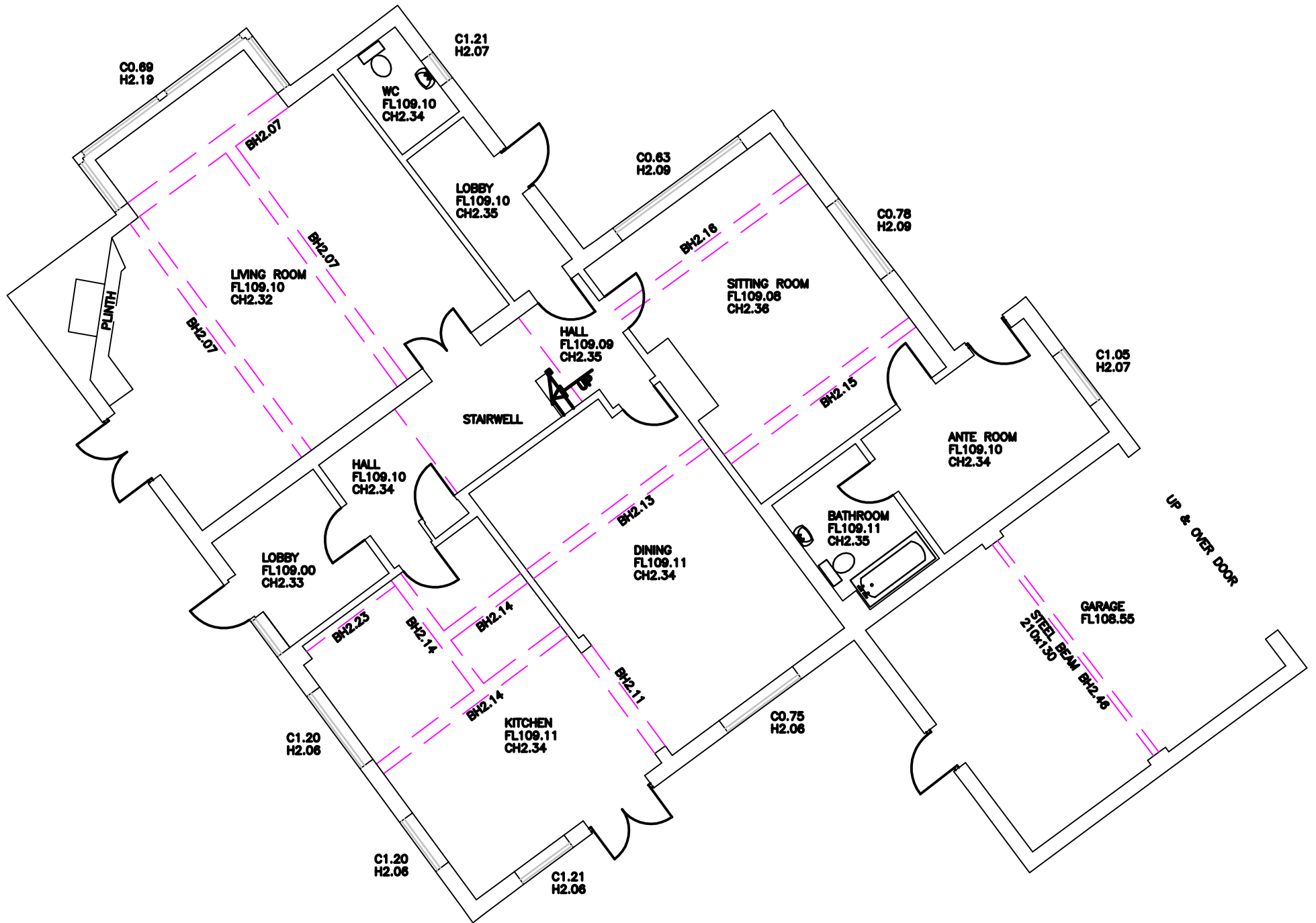
GROUND FLOOR
